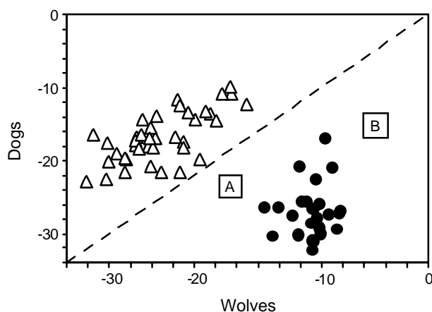
Figure 1 Log likelihood of assignment for dogs (open triangles) and Scandinavian wolves (black circles). The log likelihoods for the two target samples (A, B) are also indicated.
